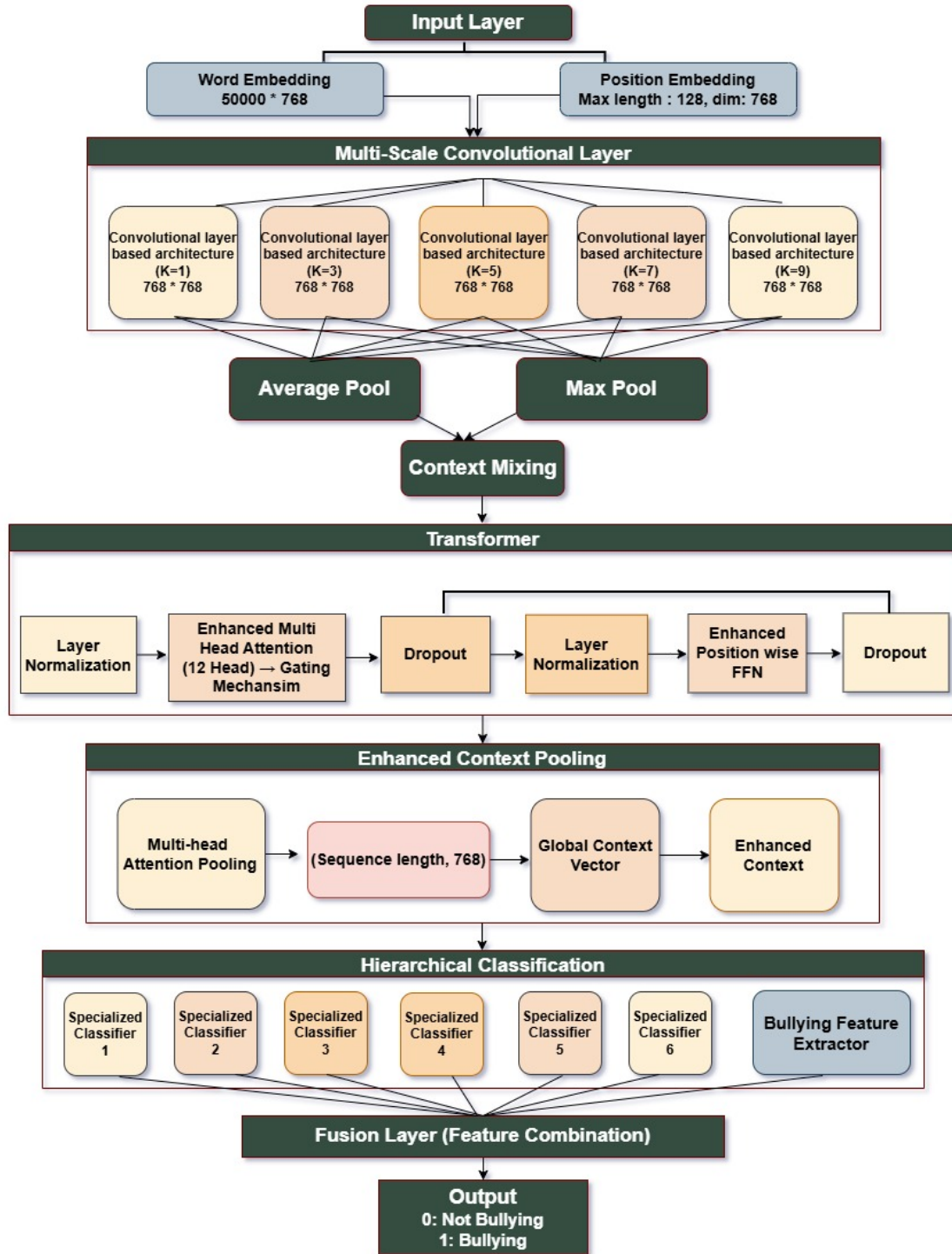
FIGURE 3.8: HighPerformanceCyberBERT architecture with multi-scale convolutional features, enhanced attention mechanisms, and hierarchical classification components
